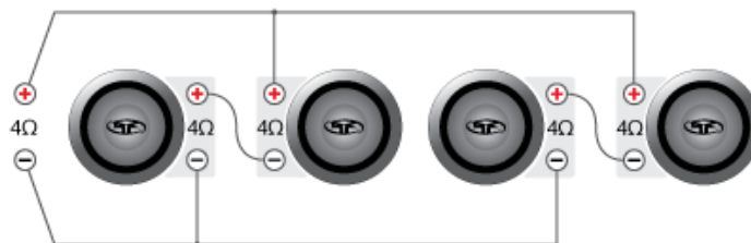
(4) 4 Ohm SVC Speakers = 4 Ohm Load
