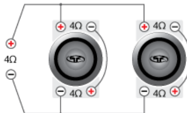
(2) 4 Ohm DVC Speakers = 4 Ohm Load
