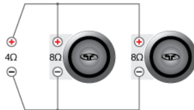
(2) 8 Ohm SVC Speakers = 4 Ohm Load
