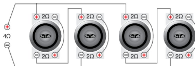
(4) 2 Ohm DVC Speakers = 4 Ohm Load
